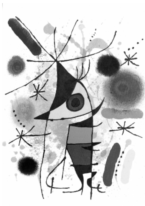
(c) Luminance
